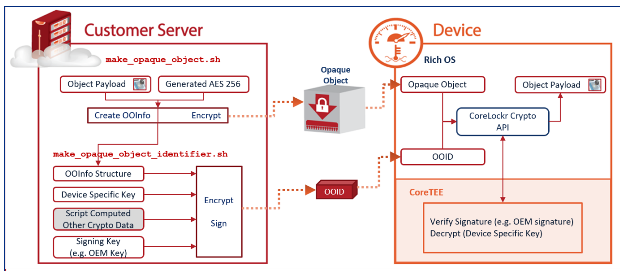
Figure 3 Opaque Objects
