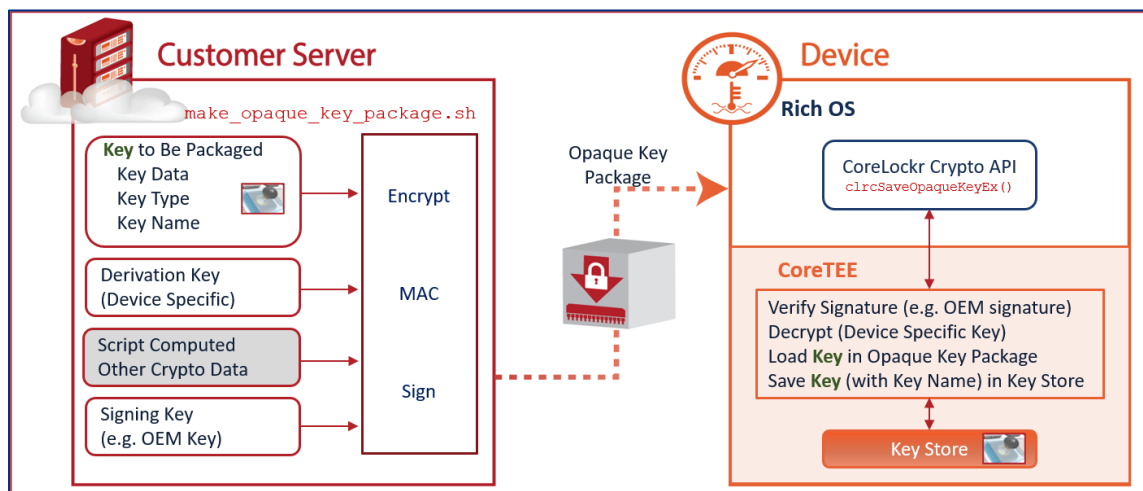
Figure 2 Opaque Keys
