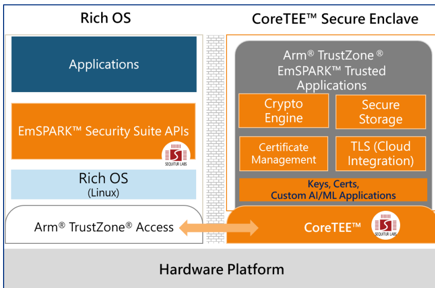
Figure 1 EmSPARK Architecture
