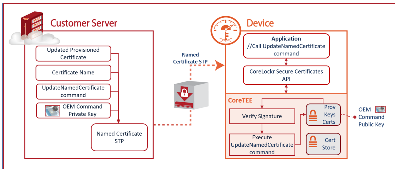
Figure 4 Provisioned Certificate Management Flow
